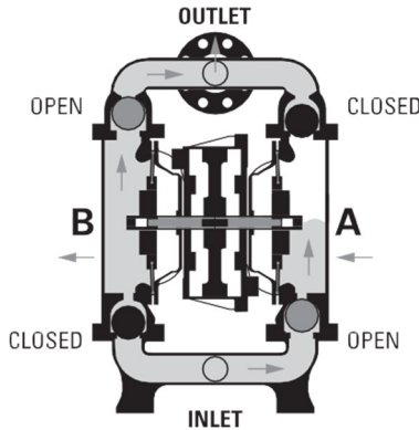
FIGURE 2 Once the shaft has reached the end of its stroke, the air valve redirects pressurized air to the back side of diaphragm B.
