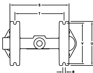
ALTERNATE FOOTPRINT
